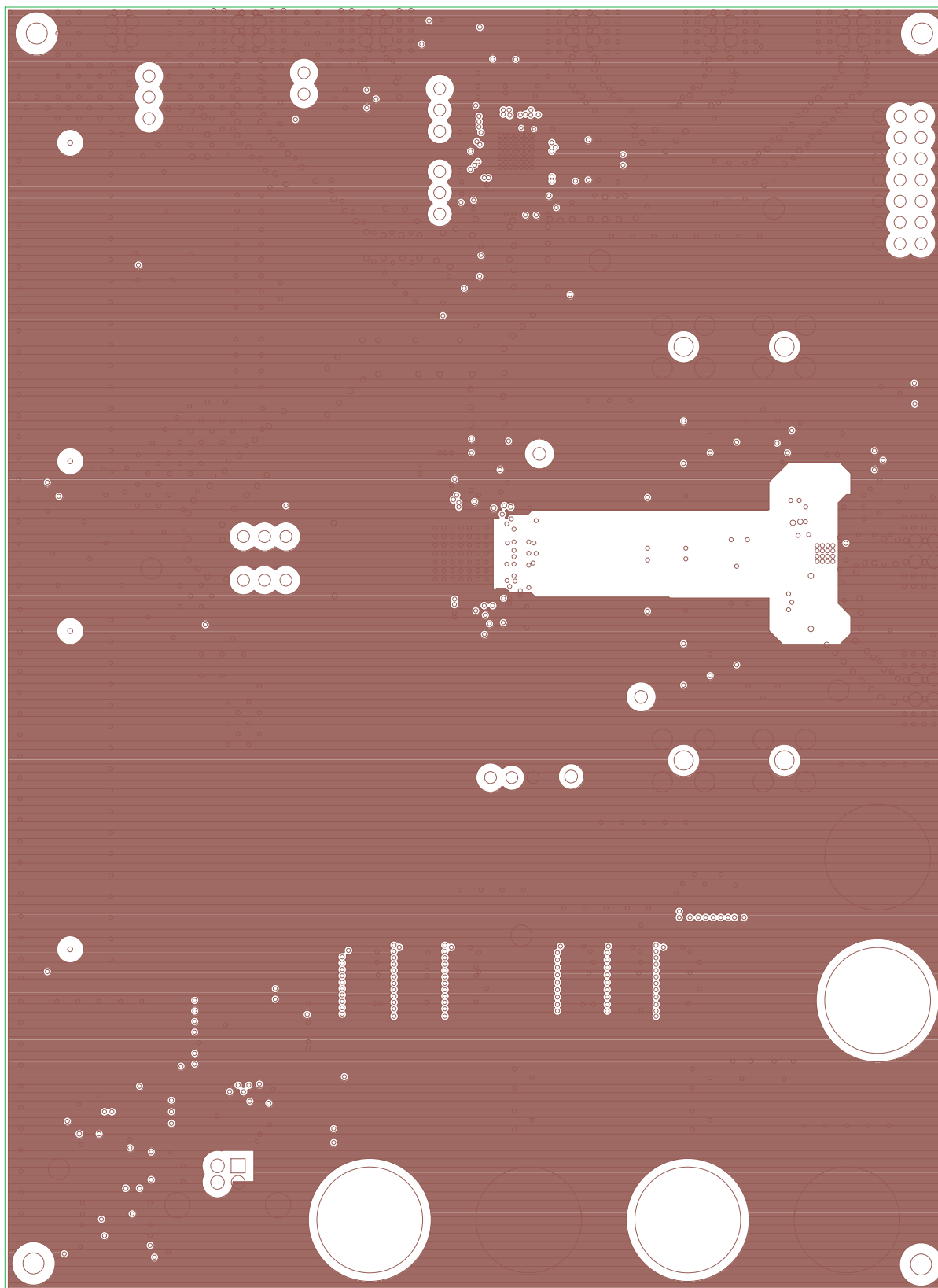
Figure 7. Layer 2, GND
