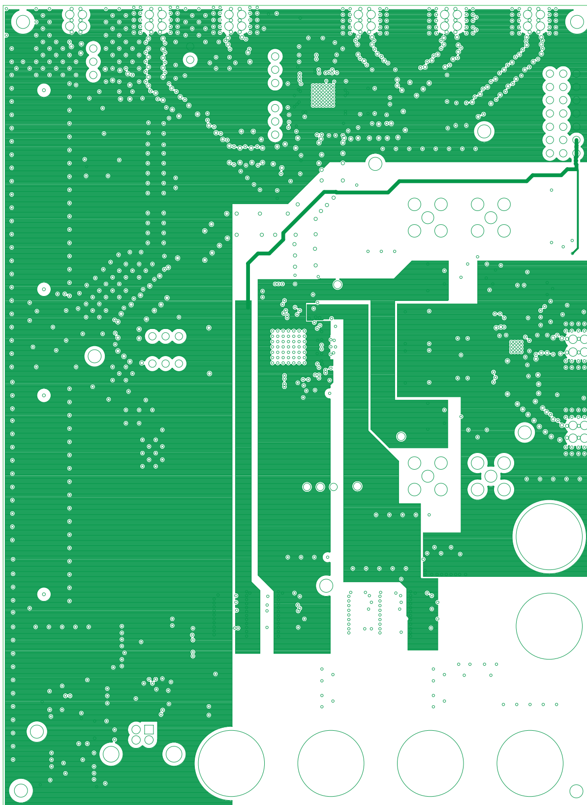
Figure 9. Layer 4, PWR
