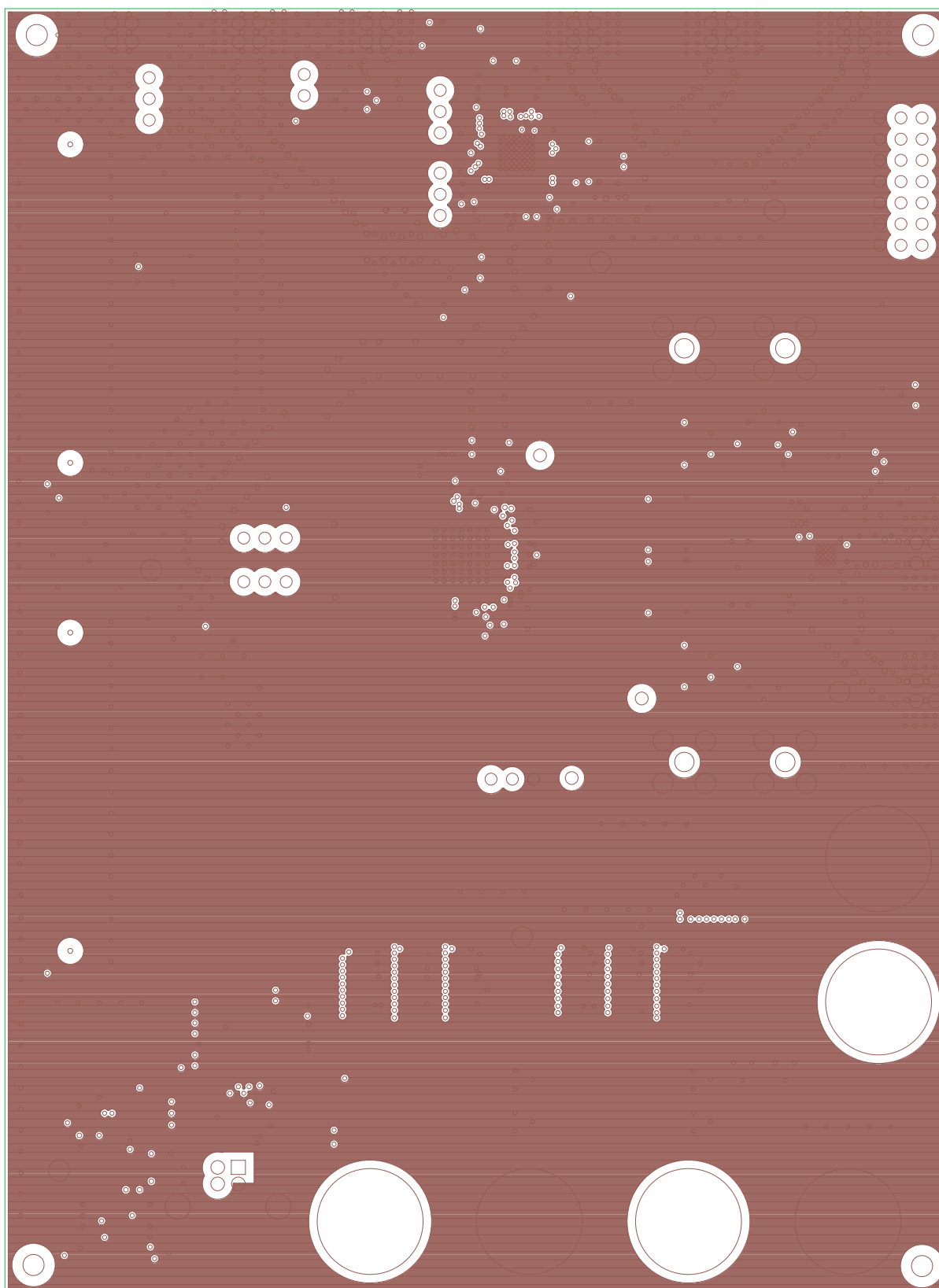
Figure 8. Layer 3, GND
