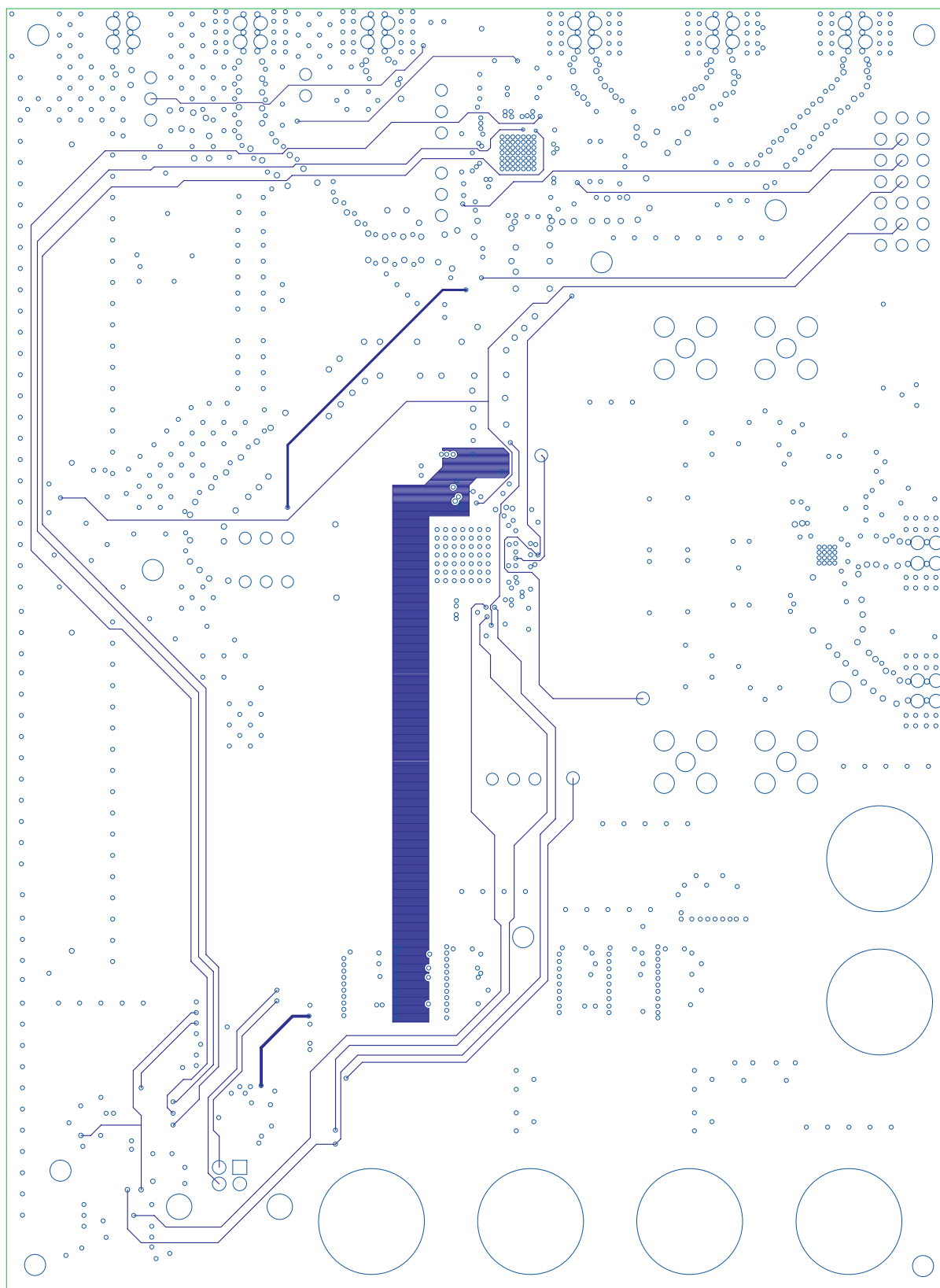
Figure 10. Layer 5
