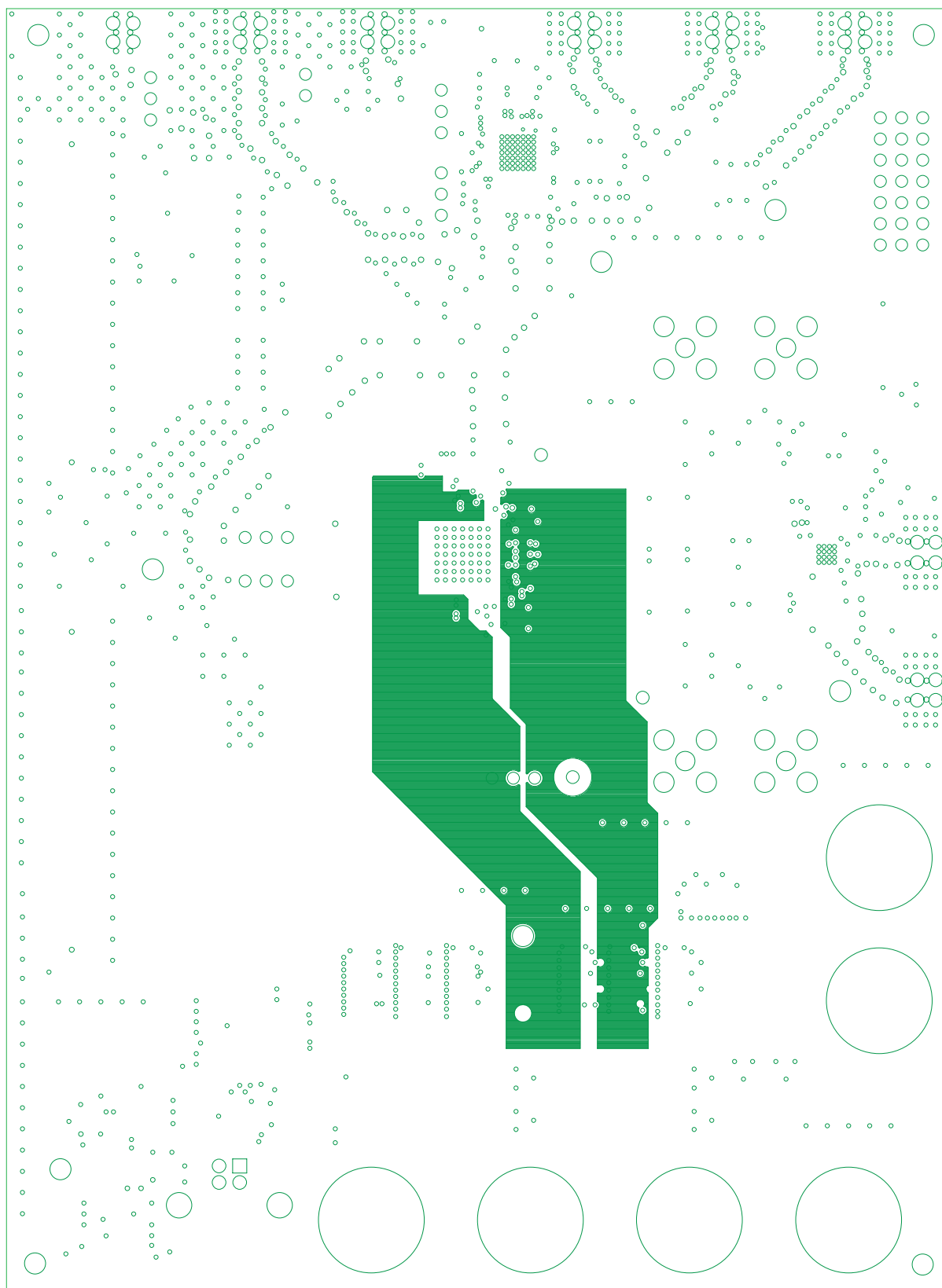
Figure 11. Layer 6, PWR
