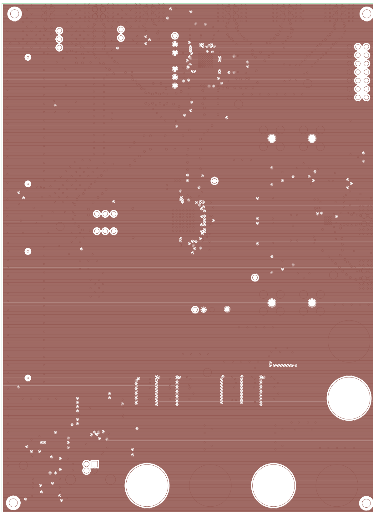
Figure 12. Layer 7, GND
